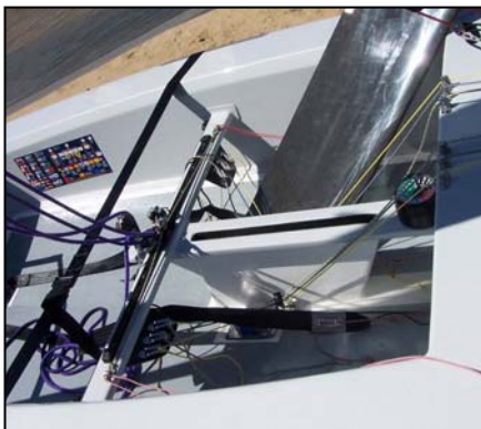
Ronstan Series 19 traveller and carbon cleat brackets
